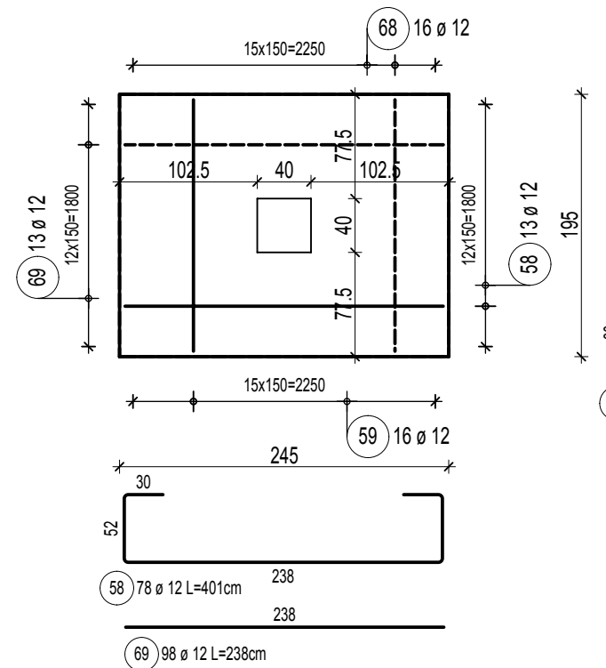
OC-5
